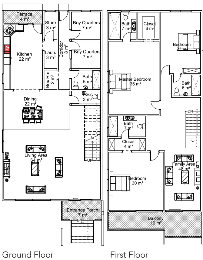
TownHouse Type B (3BR +1 MR)
